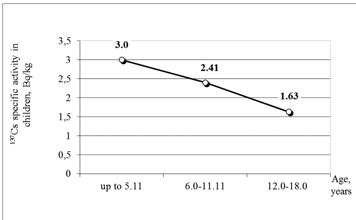
Figure. Age dependence of ^{137}\text{Cs} specific activity in a group of children from Ivankovsky and Polessky districts, Kiev region, Ukraine.
