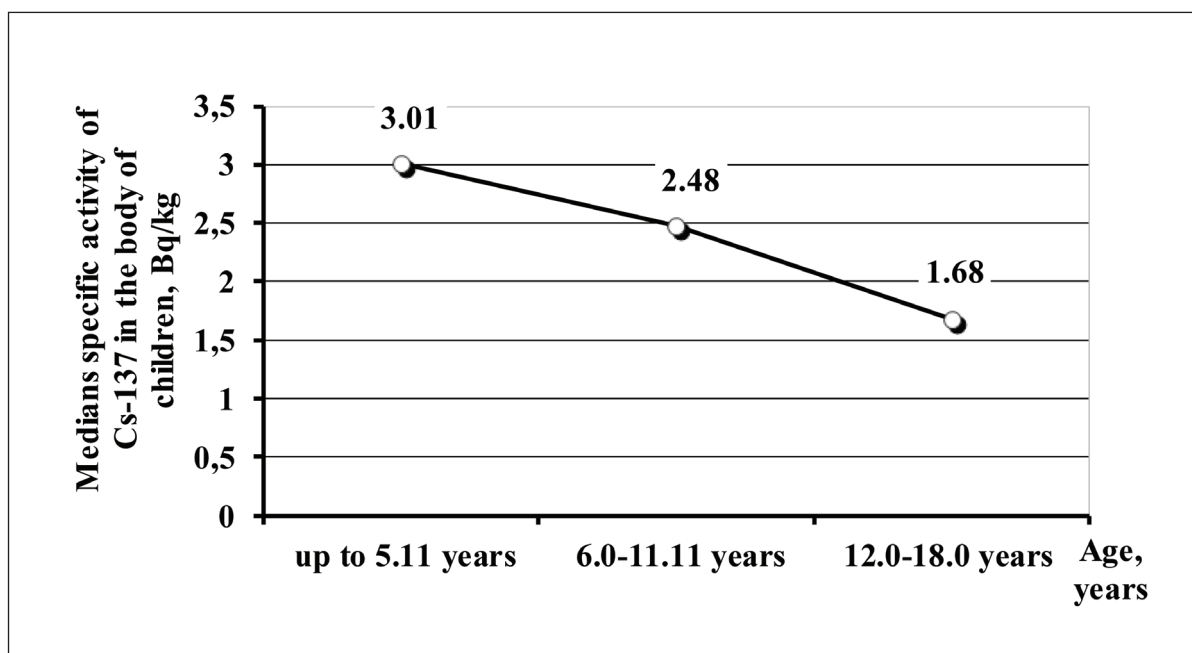
Figure. 3. The distribution of the median values of the specific activity of ^{137}\text{Cs} in the body of children of different age groups.
