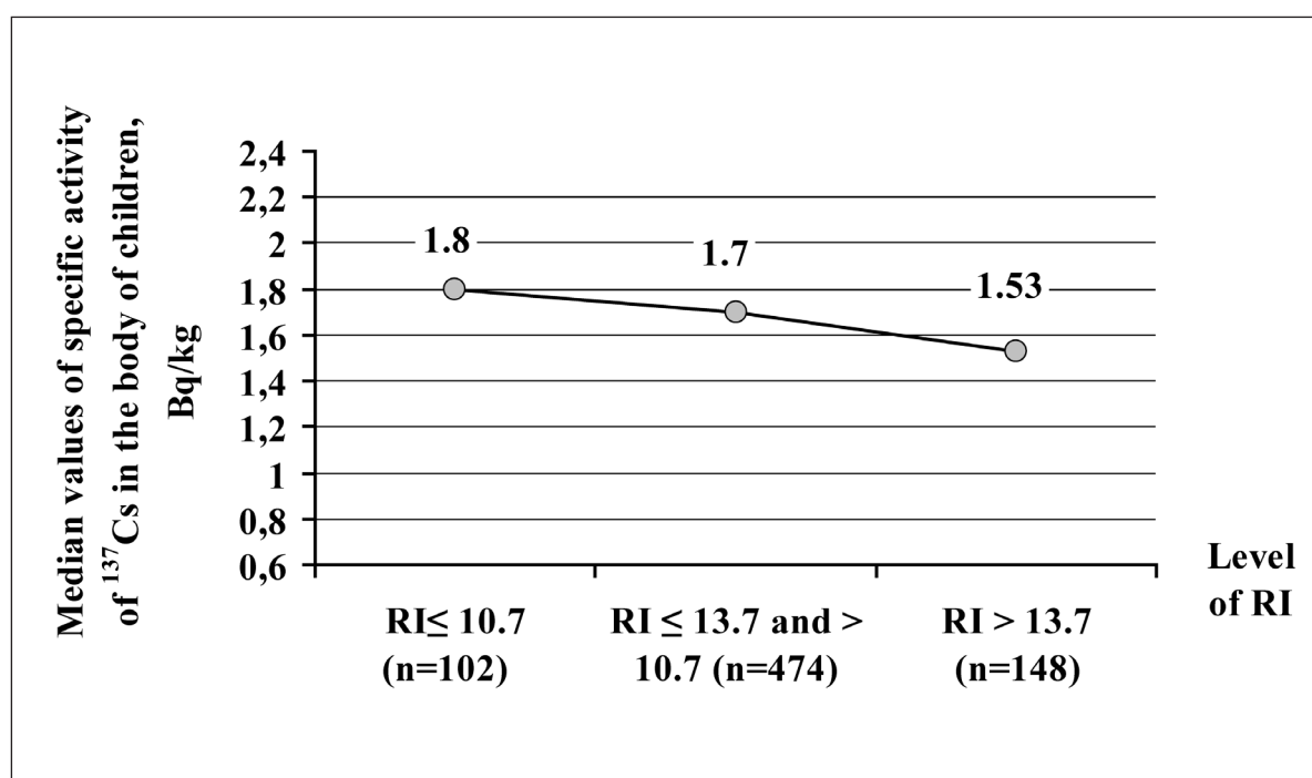
Figure. 1. Distribution of medians of ^{137}\text{Cs} specific activity values in the body of children of the older group with different levels of physical development (Rohrer index).
